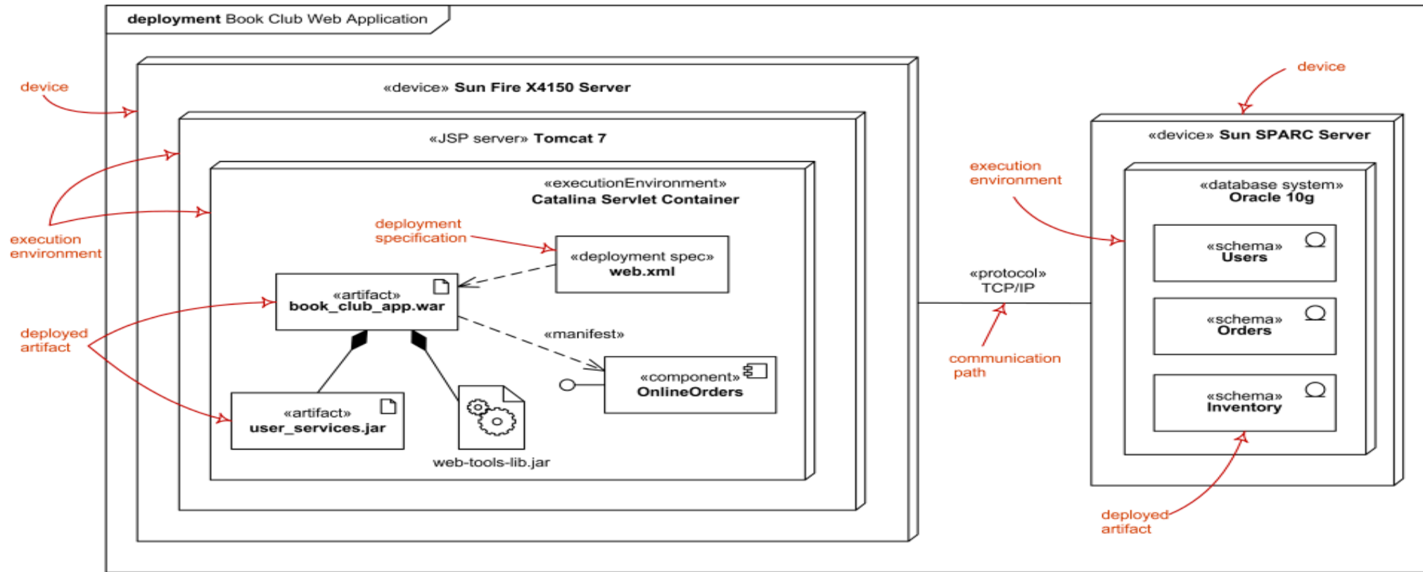
Specification level deployment diagram - web application deployed to Tomcat JSP server and database schemas - to database system
