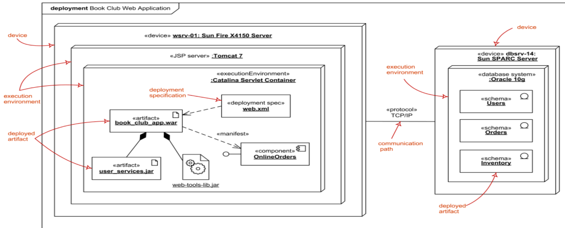
Instance level deployment diagram - web application deployed to Tomcat JSP server and database shemas - to database system
